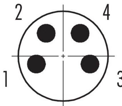
Contact arrangement (Plug-in side)
