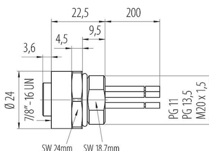
Scale drawing
