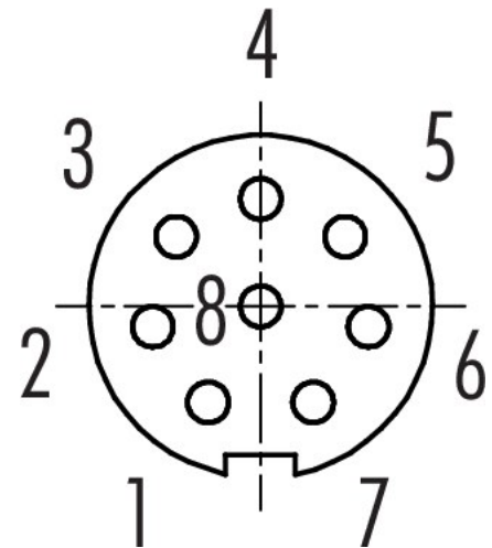
Contact arrangement (Plug-in side)
