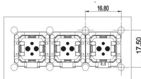
Kleinstes Raster / Minimum grid: 16.80 x 17.50
